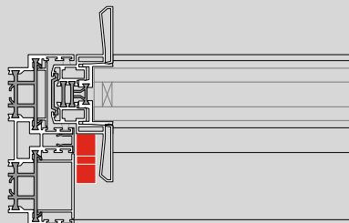
sliding | multipoint | frame coulissante | serrure multipoint | cadre
