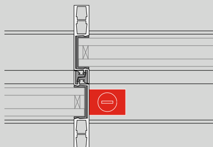
sliding | one point | central mullion coulissante | un point | profil central
